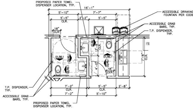
03 ENLARGED RESTROOM PLANS SCALE: 1/4" = 1'-0"
